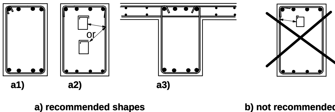
Figure 9.6: Examples of shapes for torsion links
