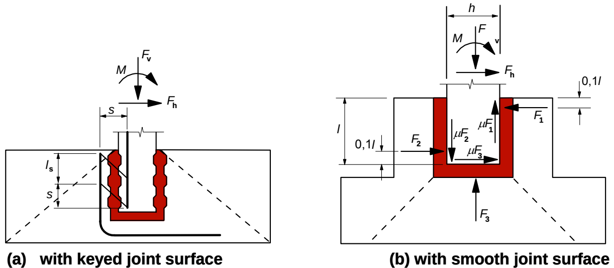
Figure 10.7: Pocket Foundations
